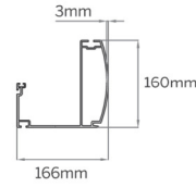
② Gutter
