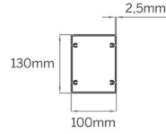
③ Post
